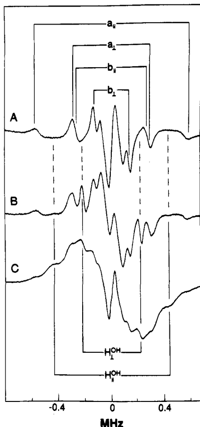
Figure 2. Proton ENDOR spectra of spin-labeled penicillin in different solvents to illustrate a tightly bound methanol molecule: (A) 50:25:25 (v/v) ^2\text{H}_6 ]DMSO: ^2\text{H}_8 ]toluene: ^2\text{H} ]chloroform to which ^2\text{H}_4 ]methanol was added in 1:1 stoichiometry with spin-labeled penicillin; (B) the same ternary solvent system to which a 1:1 molar equivalent of ^2\text{H}_3 ]methanol was added; (C) pure ^2\text{H}_3 ]methanol. These spectra were taken with \text{H}_0 at setting B of the EPR spectrum. Both parallel and perpendicular hfc components of the methanol hydroxyl proton are identified in spectra B and C. Other line pairs are assigned to H(14) and H(6), as listed in Table 2. In order to observe the new proton resonances assigned to a hydrogen-bonded methanol molecule as shown in spectrum B, it was necessary to avoid all possible sources of adsorbed moisture because of its broadening effect. All perdeuterated aprotic solvents were of highest grade ( \geq 99.6\% ^2\text{H} ), and vials of solvents were freshly opened only immediately prior to use. Acid-washed EPR sample tubes were kept in a desiccator at least overnight prior to use, and samples were prepared under nitrogen and immediately frozen and stored in liquid nitrogen until use.
