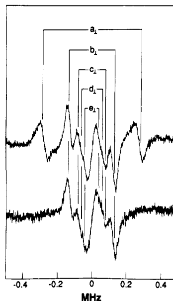
Figure 1. Proton ENDOR spectra of spin-labeled penicillin in 50:50 (v/v) [ 2 H 6 ]DMSO:[ 2 H 4 ]methanol. The static magnetic field was at setting A of the EPR spectrum. For the top spectrum, the sample was first dissolved in DMSO and then rapidly mixed with [ 2 H 4 ]methanol and frozen in liquid nitrogen. The bottom spectrum was obtained after thawing the sample to allow exchange of the amide proton H(14). Four other line pairs are identified in the stick diagram and are assigned to the perpendicular hfc components of specific protons (see text). The abscissa indicates the ENDOR shift (measured ENDOR frequency minus free proton Larmor frequency).
